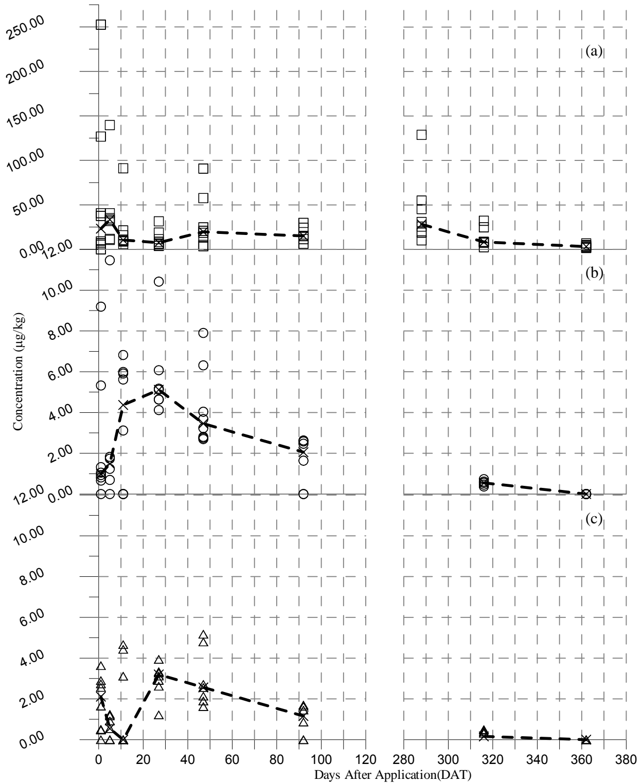
Figure 4.1. 2,4-D concentration measured in surface (a, 0-7.5 cm), root zone (b, 10-30 cm), and below root zone (c, 36-60 cm) soil at the Delta Junction site. The trend lines in each plot represents the median sample concentration. Herbicide was applied to the site on July 6, 2006. The soil froze approximately 120 days after application and thawed approximately 286 days after application. The break in the ordinate axis represents this frozen period. Note the concentration scale difference between (a) and both (b) and (c).
