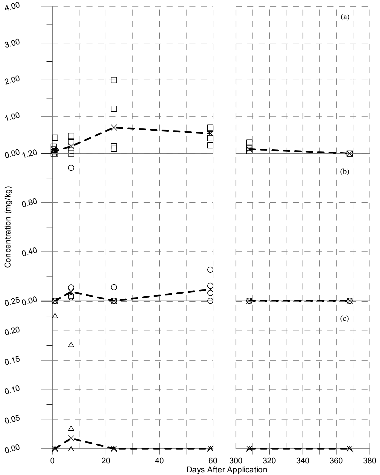
Figure 5.3. Triclopyr concentration measured in surface (a, 0-7.5 cm), root zone (b, 10-30 cm), and below root zone (c, 36-60 cm) soil at the Valdez site – Plot 12. The trend line in each plot represents the median sample concentration. Herbicide was applied to the site on July 6, 2006. Note the concentration scale difference in the three graphs.
